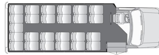
25 Passenger with Driver 4 Passenger Foldaway Seats Plus Driver
