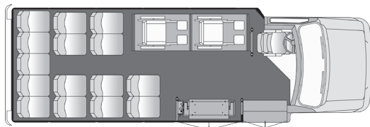
15 Passenger 2 Wheelchair with Front Lift Plus Driver
