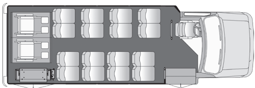
16 Passenger 2 Wheelchair with Rear Lift Plus Driver 4 Passenger Foldaway Seats Plus Driver
