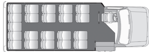
21 Passenger Plus Driver 4 Passenger Foldaway Seats Plus Driver
